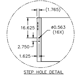
STEP HOLE DETAIL
