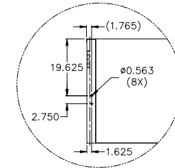
STEP HOLE DETAIL
